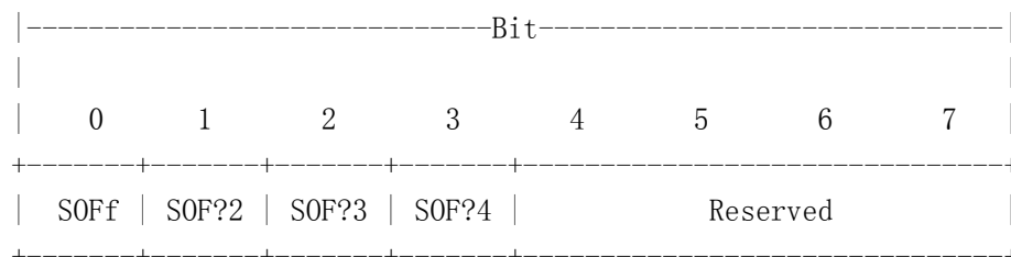
Fig. 10 Connection Usage Flags Field Format
