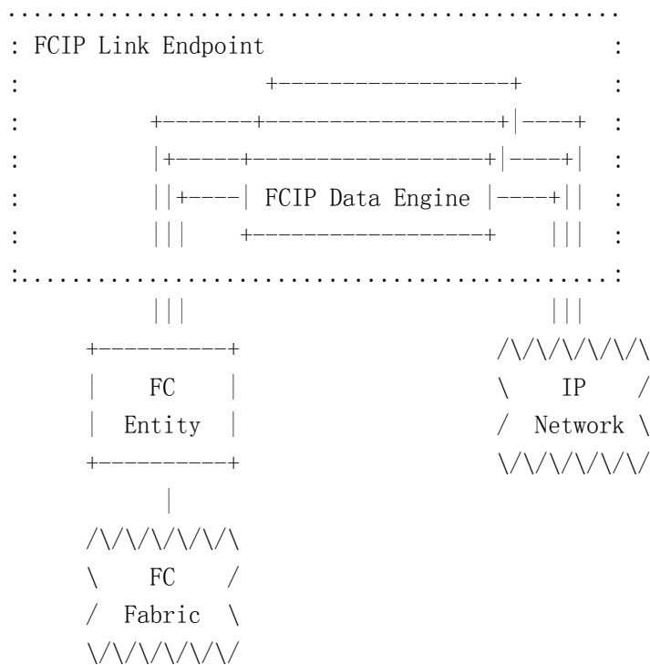
Fig. 5 FCIP Link Endpoint Model
