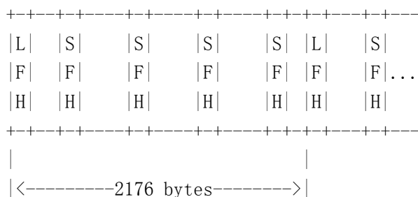
Fig. 14 Example of resynchronization data stream
