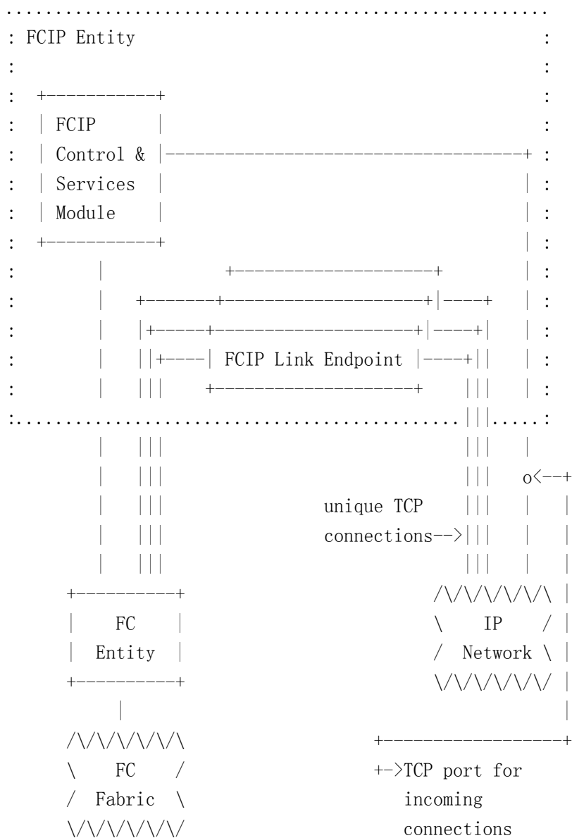
Fig. 4 FCIP Entity Model
