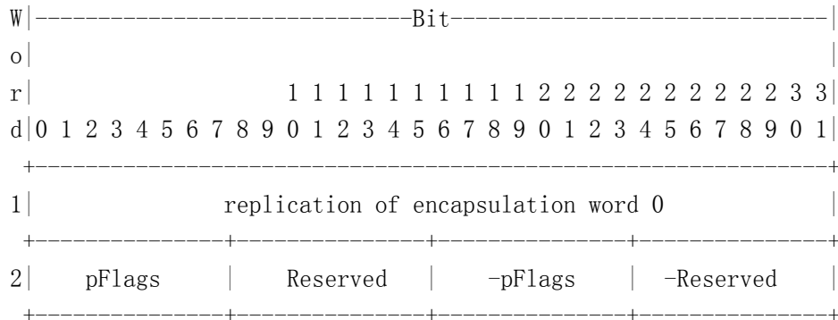
Fig. 7 FCIP Usage of FC Frame Encapsulation Protocol Specific field
