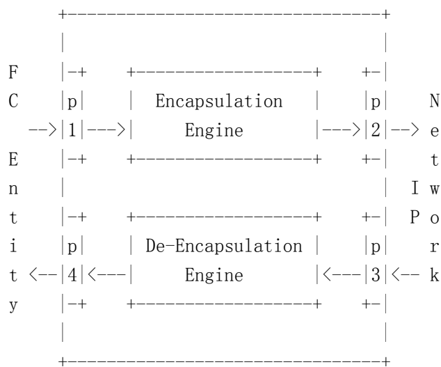
Fig. 6 FCIP Data Engine Model
