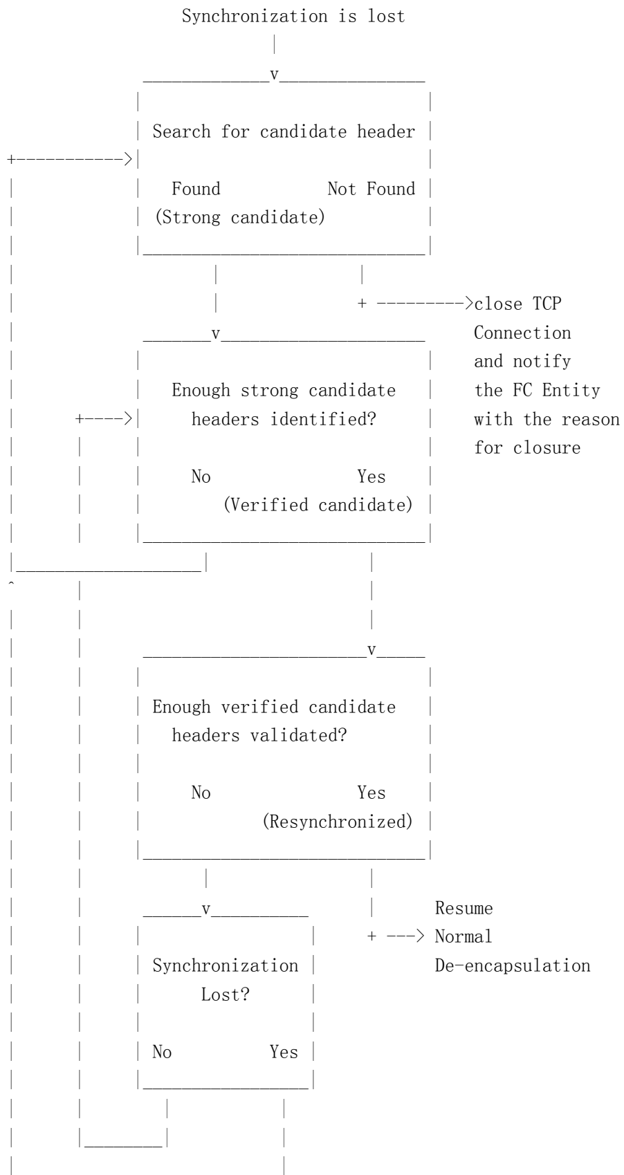
Fig. 15 Flow diagram of simple synchronization example
