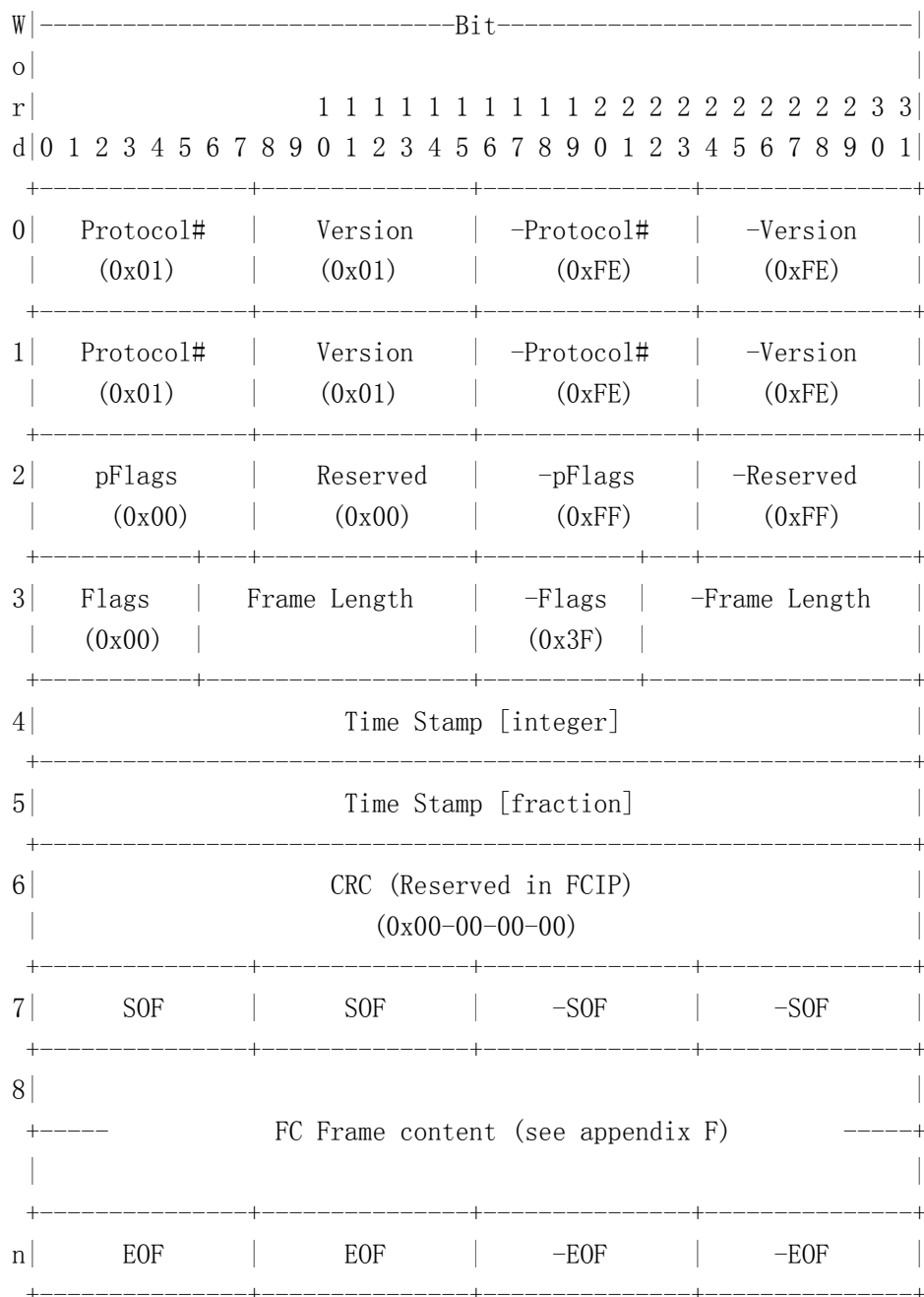
Fig. 17 FCIP Frame Format
