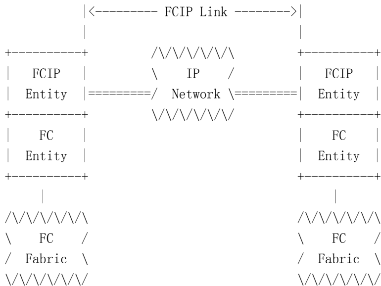
Fig. 3 Model for Two Connected FC/FCIP Entity Pairs
