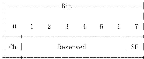
Fig. 8 pFlags Field Bits
