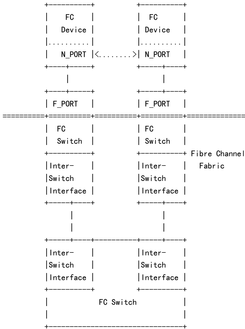
Figure 2 -- Multi-Switch Fibre Channel Fabric
