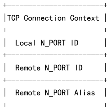
Figure 11 -- iFCP Session Descriptor
