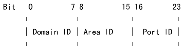
Figure 5 -- Fibre Channel Address Format
