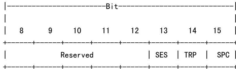
Figure 14 -- iFCP Flags Word
