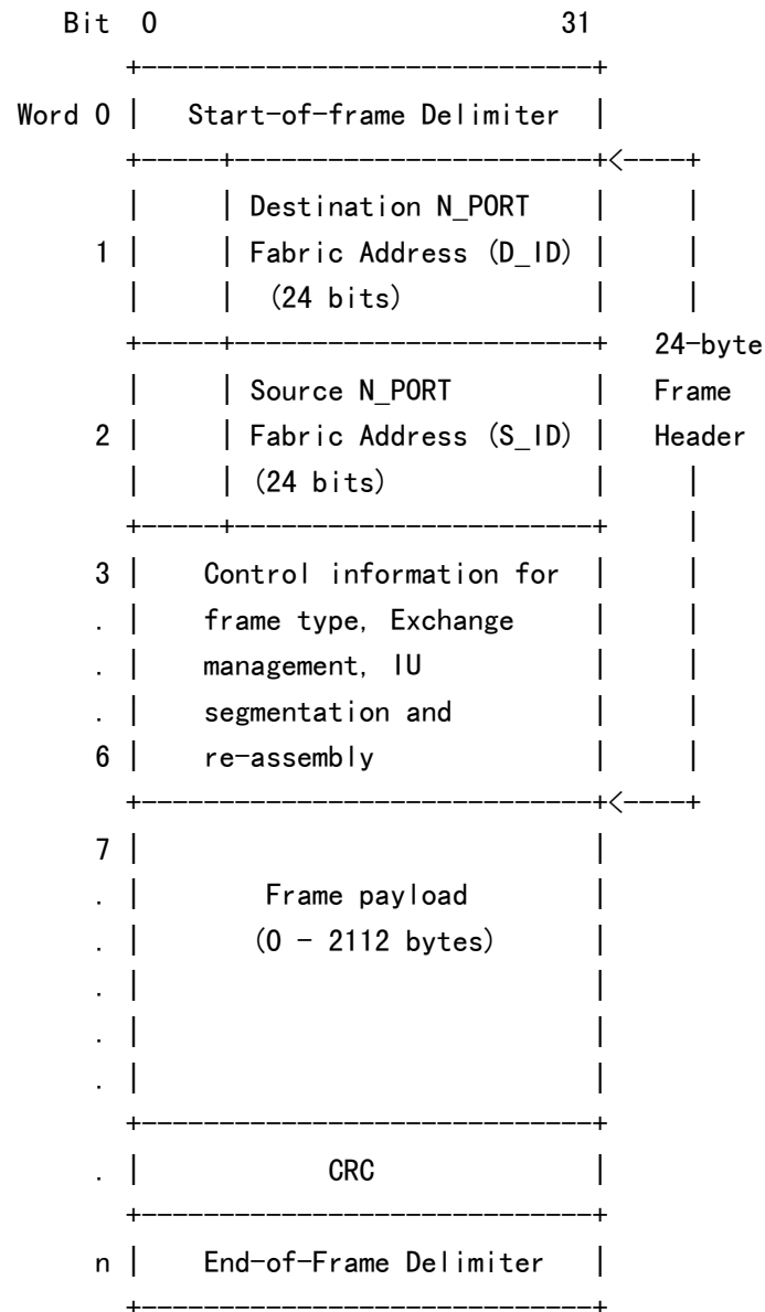
Figure 4 -- Fibre Channel Frame Format
