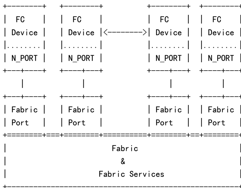
Figure 1 -- A Fibre Channel Network
