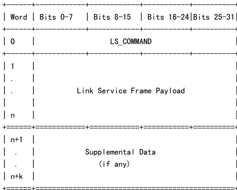
Figure 20 -- Special Link Service Frame Payload
