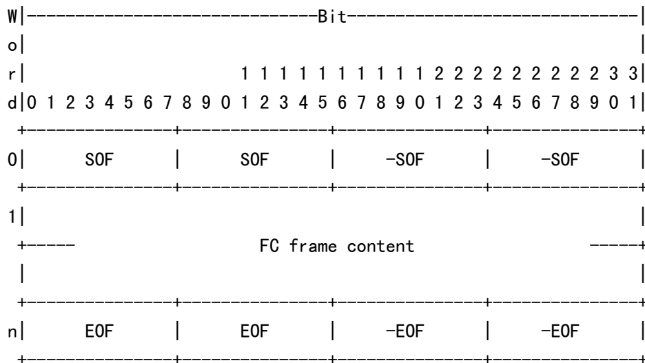
Figure 16 -- FC Frame Encapsulation Format
