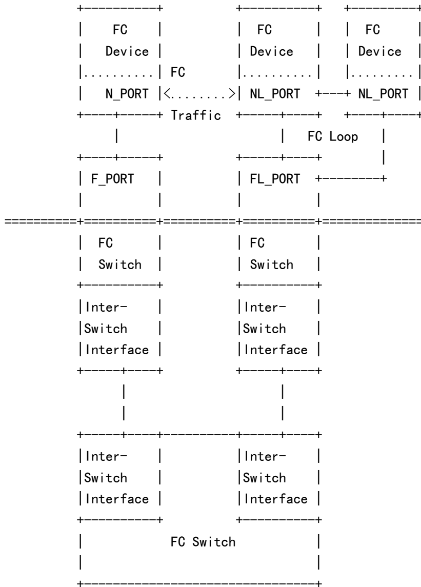
Figure 3 -- Mixed Fibre Channel Fabric
