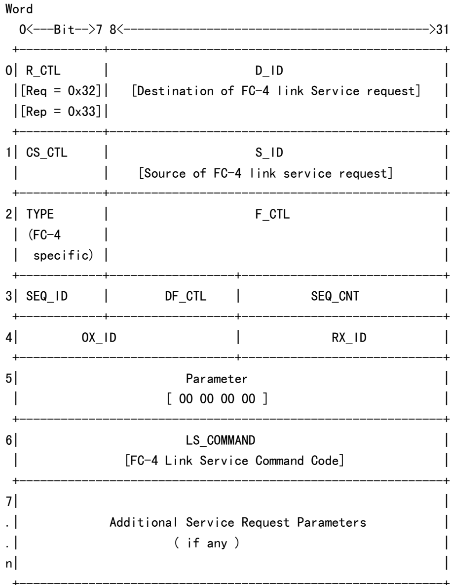
Figure 19 -- Format of an FC-4 Link Service Frame
