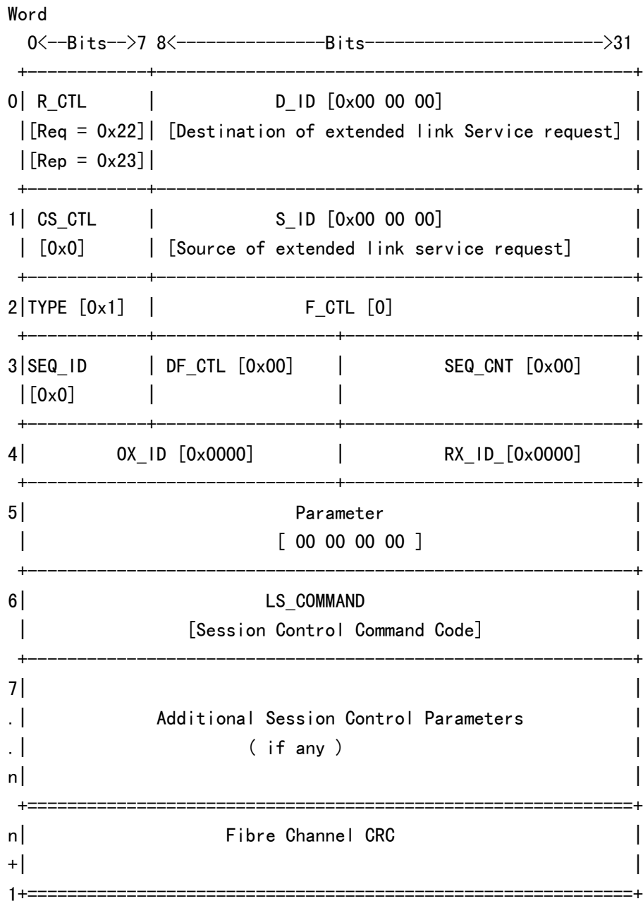
Figure 17 -- Format of Session Control Message
