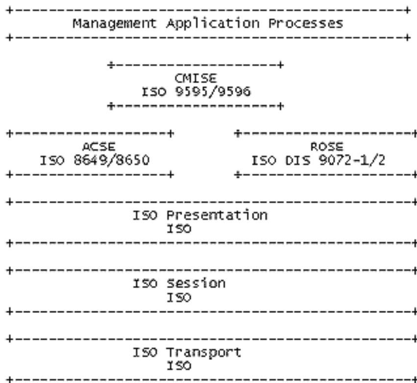
Figure 3. The CMIP Protocol Suite
