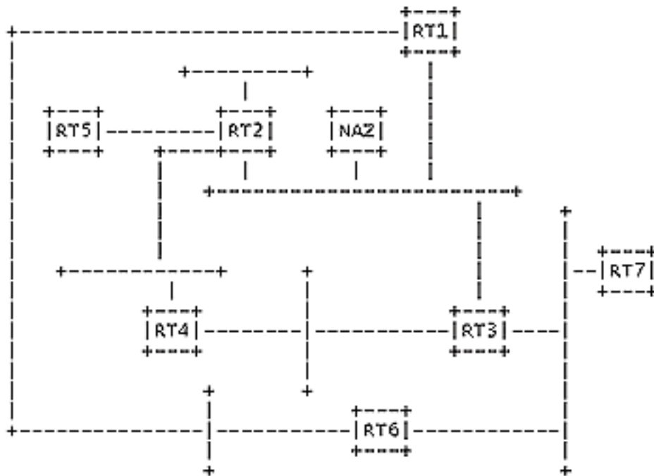
Figure 1: Initial MOSPF test setup
