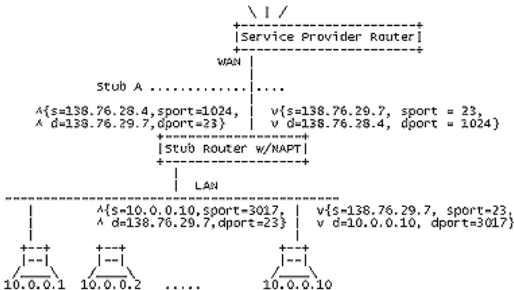
Figure 3: Network Address Port Translation (NAPT) Operation
