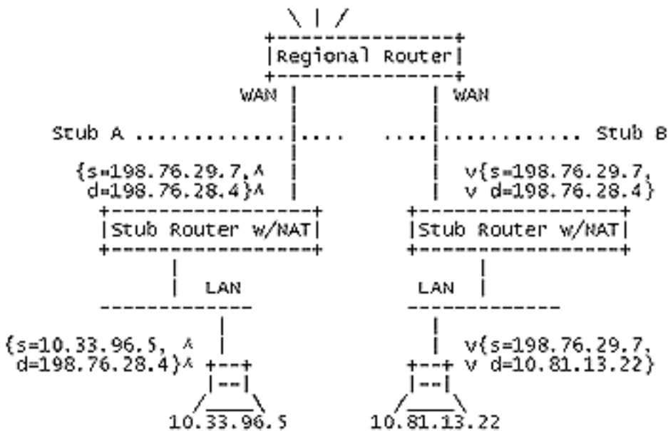
Figure 2: Basic NAT Operation
